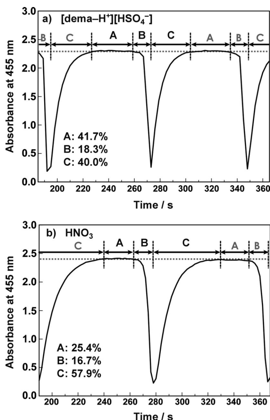
Figure 4. Waveform analysis of the BZ self-oscillation for systems using a) [\text{dema-H}^+][\text{HSO}_4^-] and b) \text{HNO}_3 as proton source.
